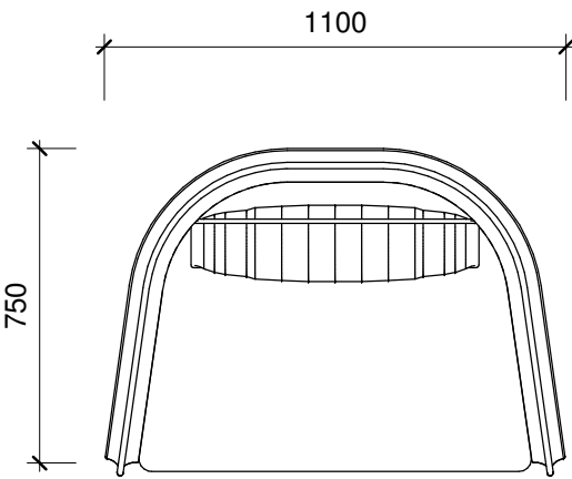
CLOUD PLAIN 1.5 HIGH
