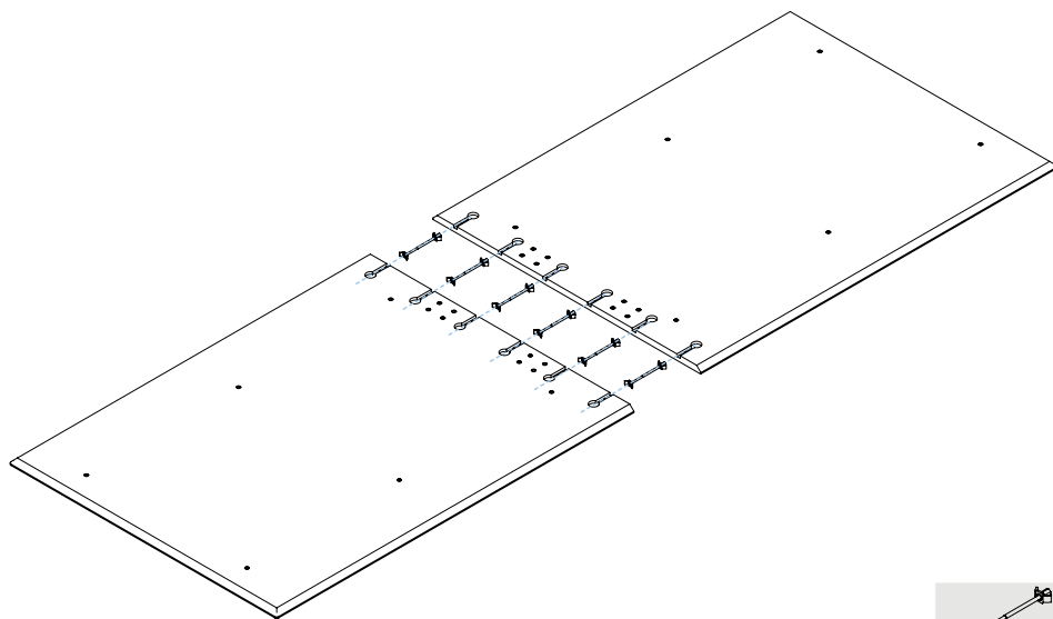
WORKTOP BOLT
